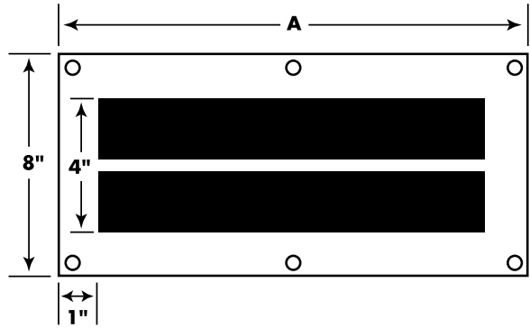
Model TG - Light Duty Plate Magnets
