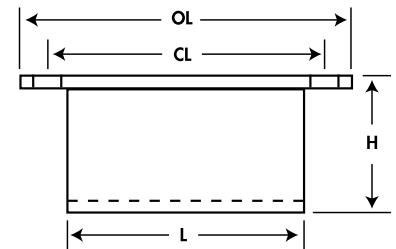
Type A Front View
